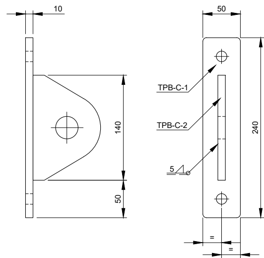
PART TPB-C Scale 1:5
