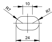
SLOTTED HOLE DETAIL Scale 1:2
