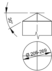
DETAIL A - TIMBER POLE TOP Scale 1:20
