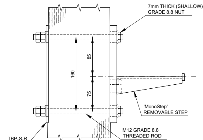
DETAIL F - REMOVABLE CLIMBING STEPS Scale 1:5
