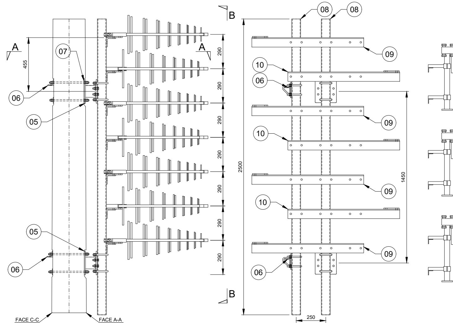
DETAIL G - Tx ANTENNA MOUNT SCALE 1:20
