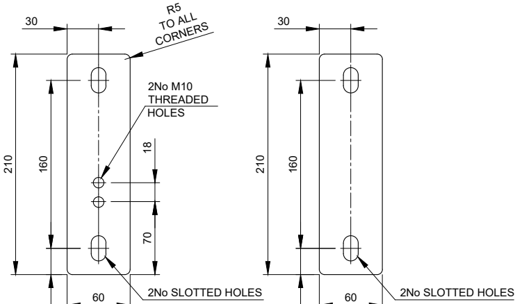
PART TPS-R-1 Scale 1:5
