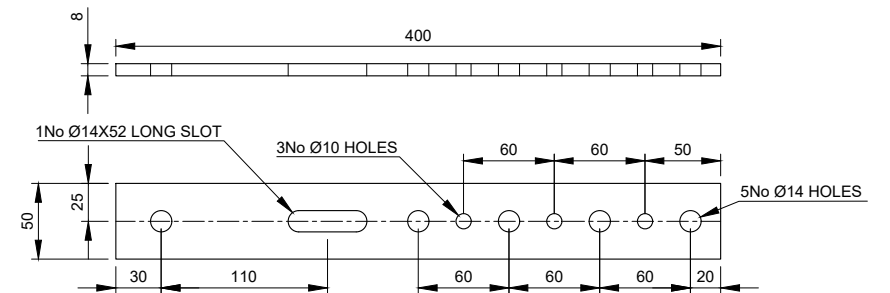
TPA-PD - 8mm THICK Scale 1:5
