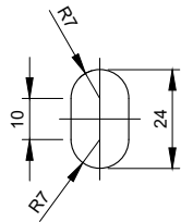
SLOTTED HOLE DETAIL Scale 1:2
