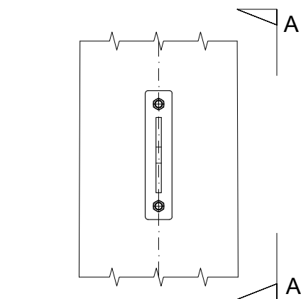
DETAIL C - FALL ARREST ATTACHMENT POINT Scale 1:10
