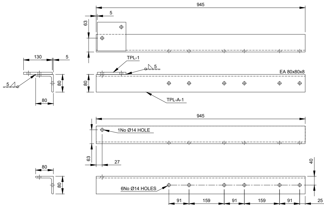
TPL-A-1 - EA 80x80x8 Scale 1:10
