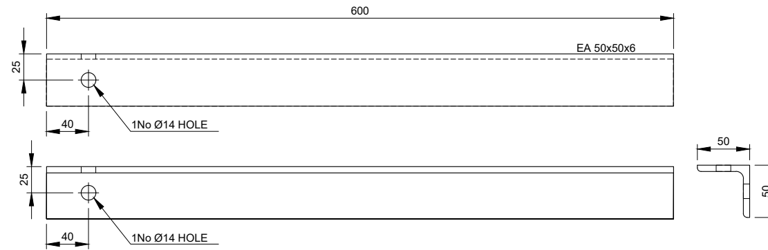
TPB-BR-1 - EA50x50x6 Scale 1:5
