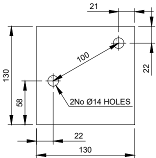
TPL-1 - 10mm THICK Scale 1:5
