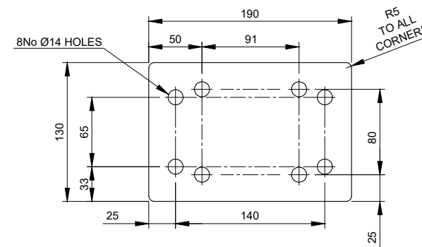
TPB-BR-3 - 10mm THICK Scale 1:5
